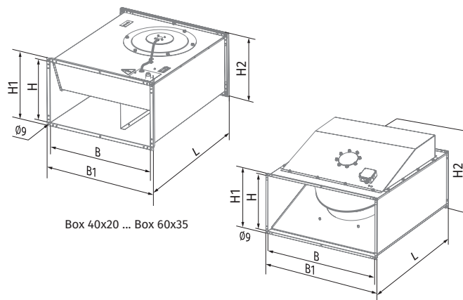
Box 100x50 4D
